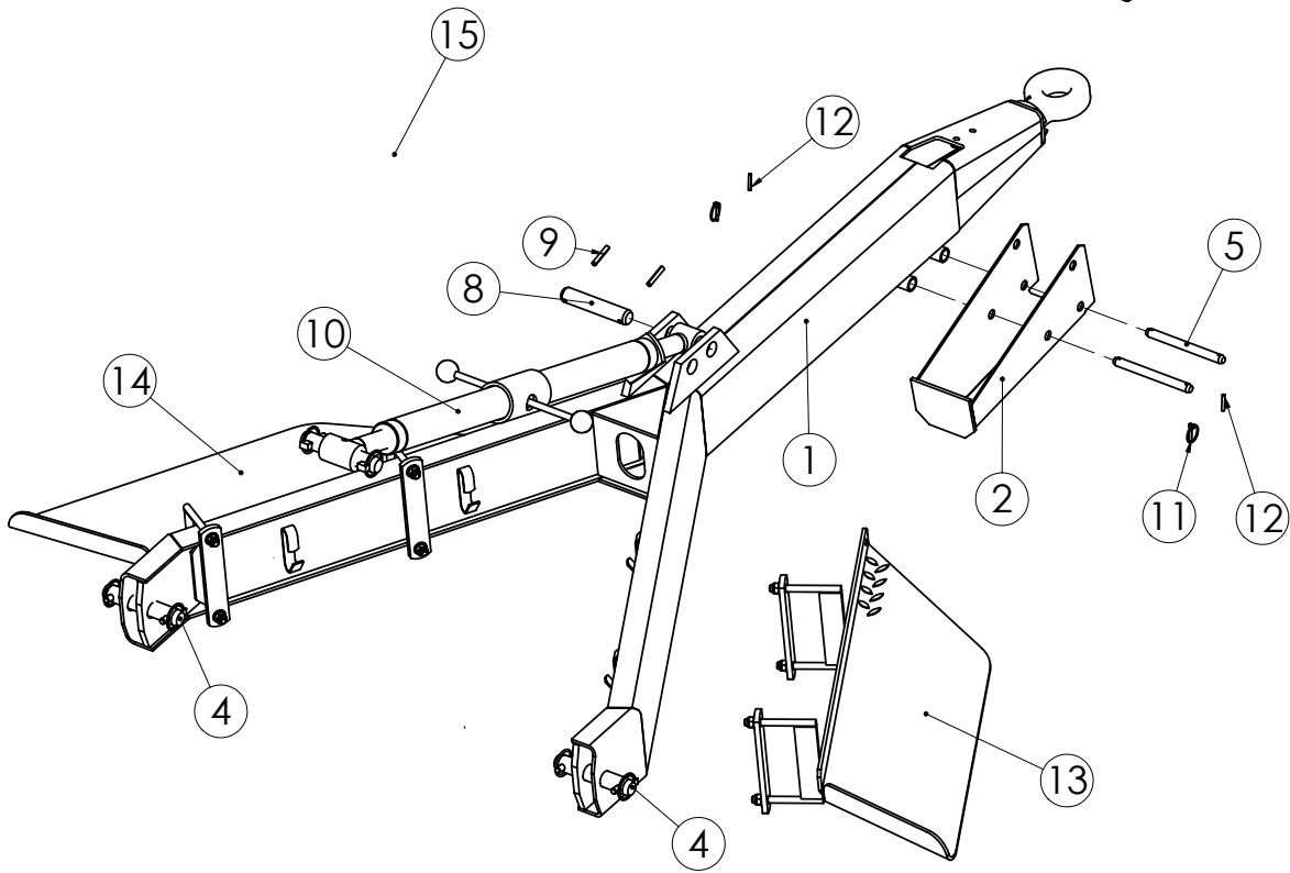
98627202 VETOLAITE KP.
