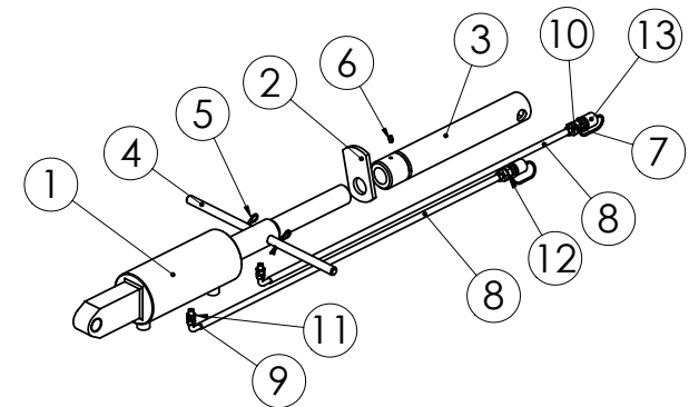
AISASYLINTERI 98635603
