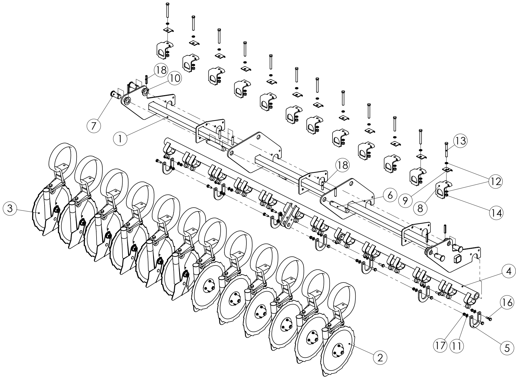
98703102 LASERVANNASRUNKO KP. 3000
