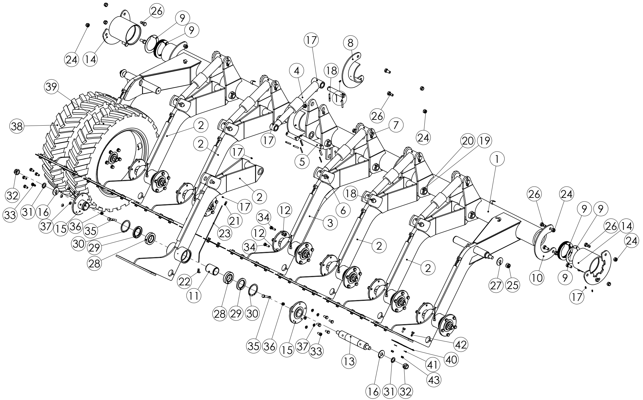
99072002 Wheel set TITAN 4000
