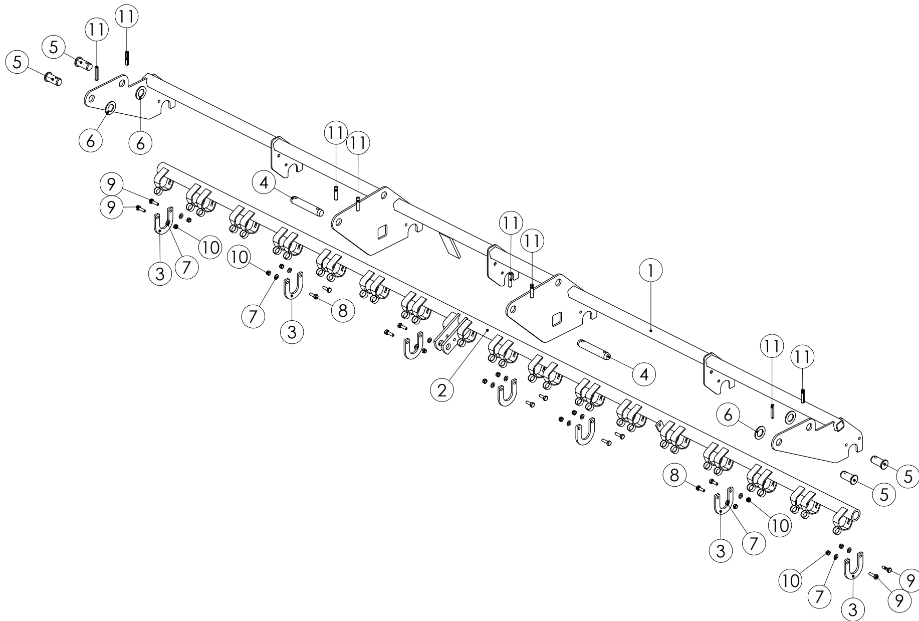
98979002 ETUVANNASRUNKO 4000
