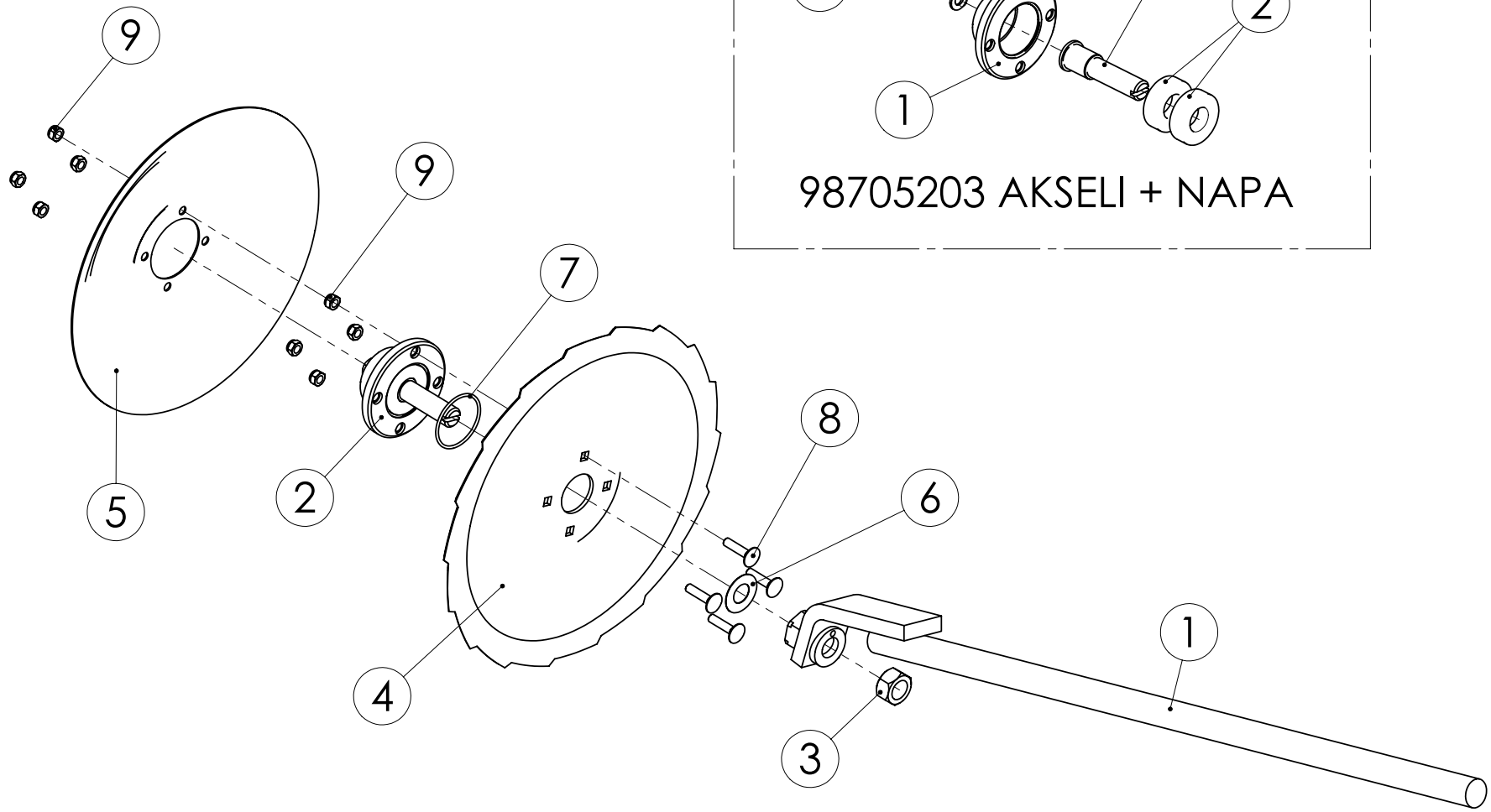
98683503 LAUTANEN+VARSI, VASEN
