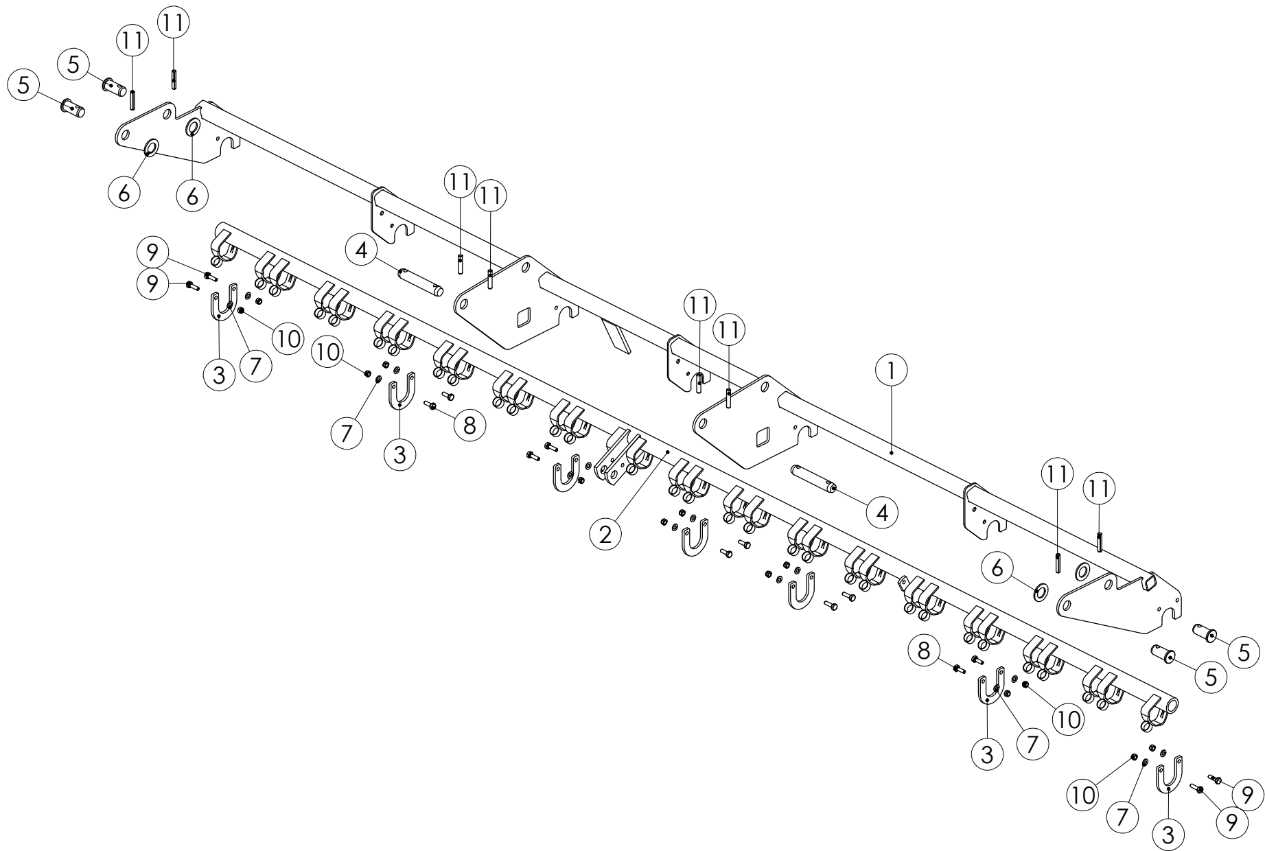
98979002 ETUVANNASRUNKO 4000
