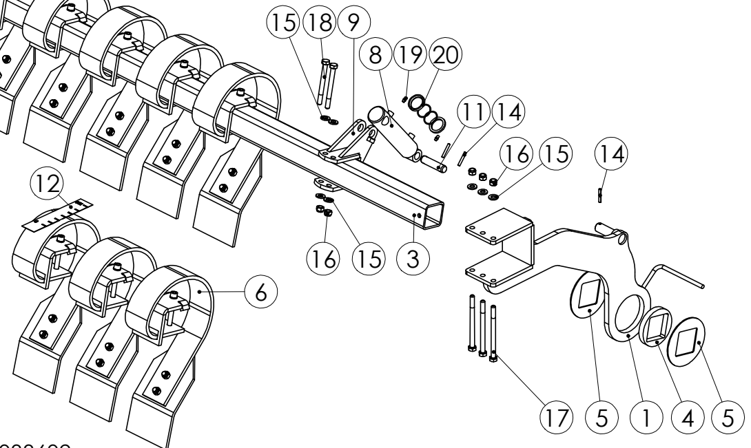
99033602 ETULATA KP. 4000 Levelling board assembly 4000 Frontsladd aggregatet 4000
