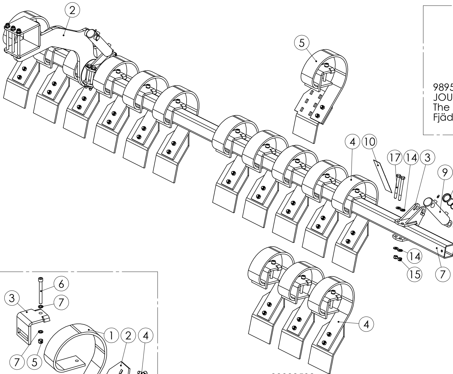
99033502 ETULATA KP. 3000 Levelling board assembly 3000 Frontsladd aggregatet 3000
