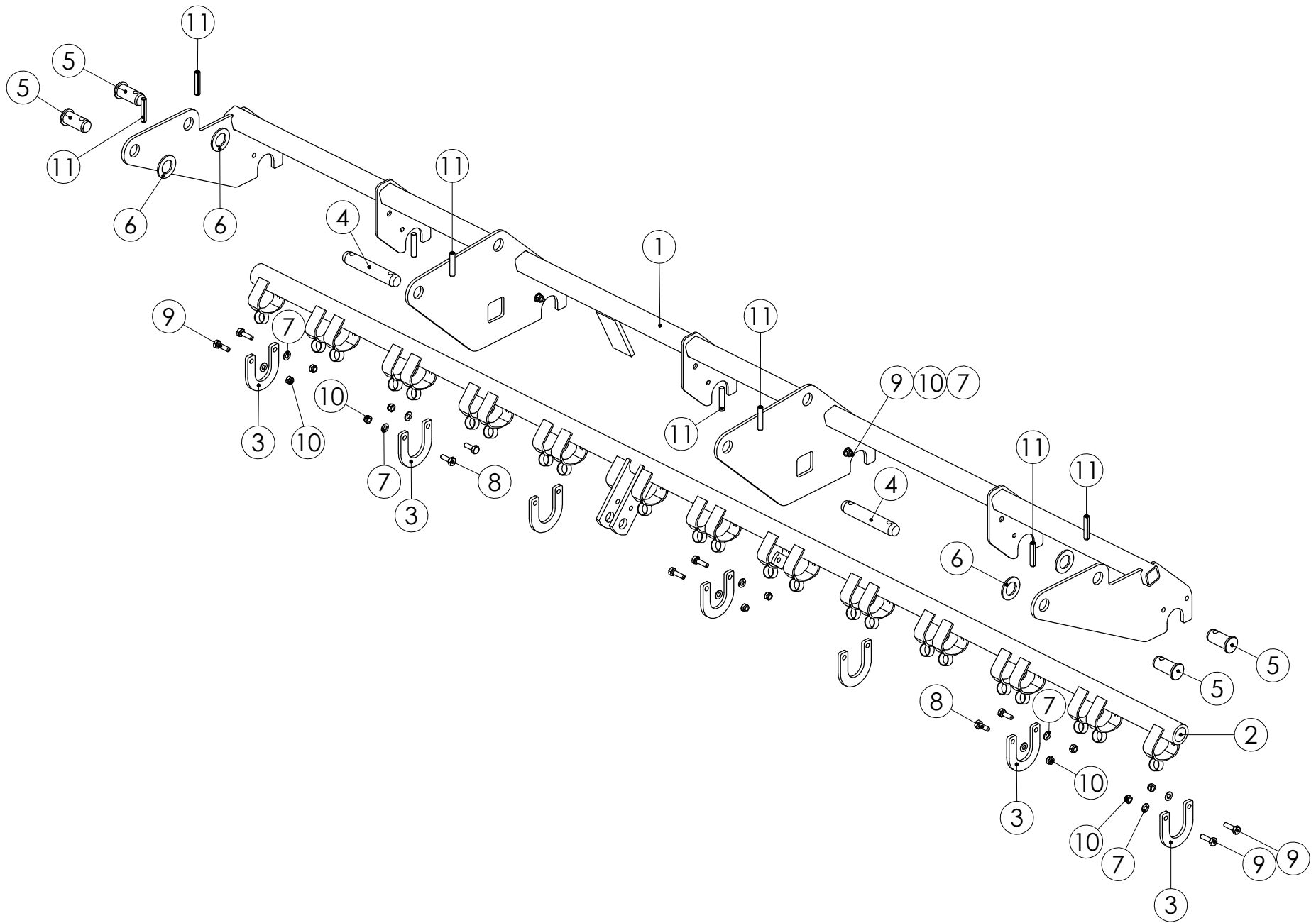
98981802 ETUVANNASRUNKO KP. 3000
