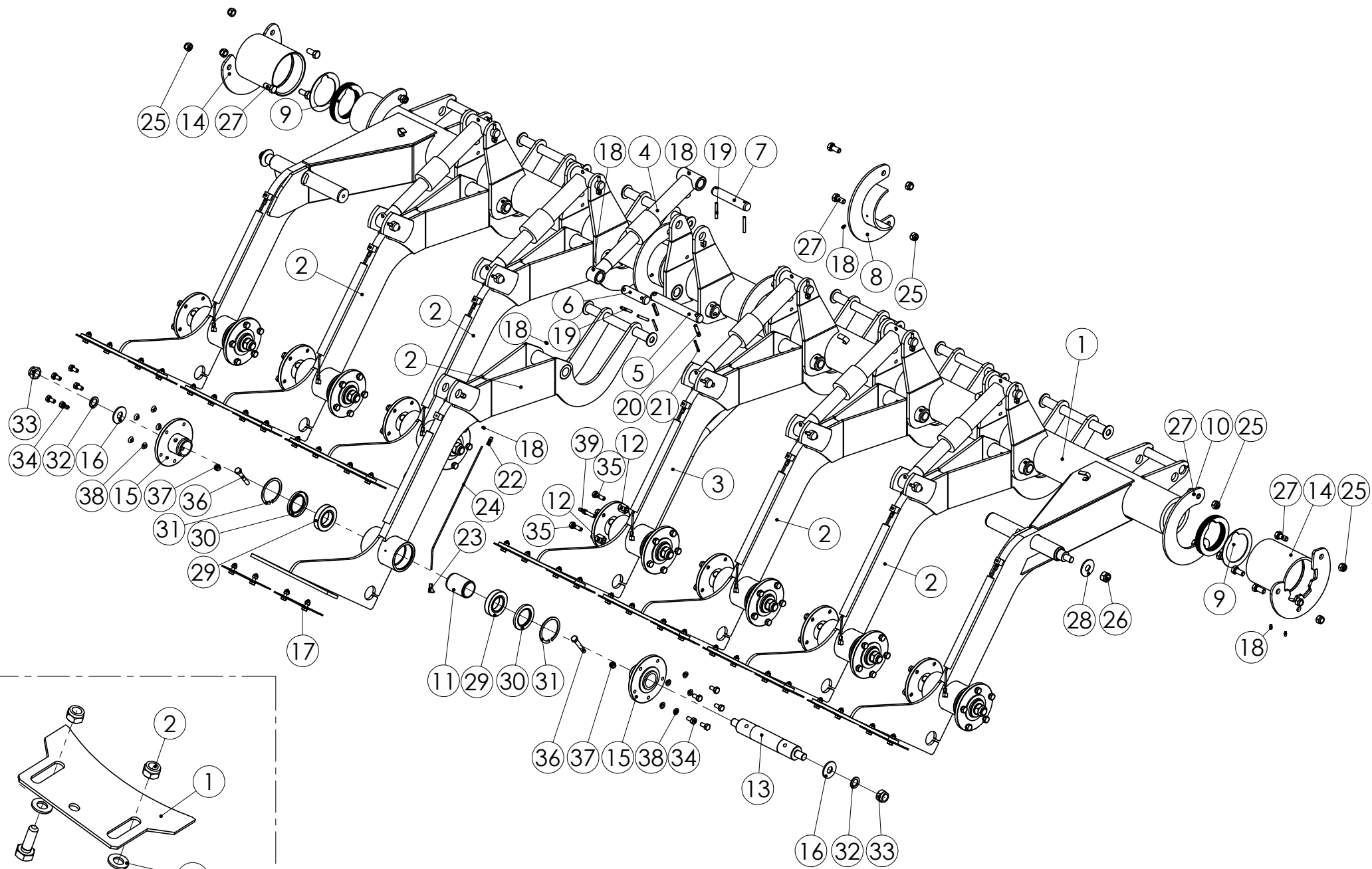
98348004 Scraper
