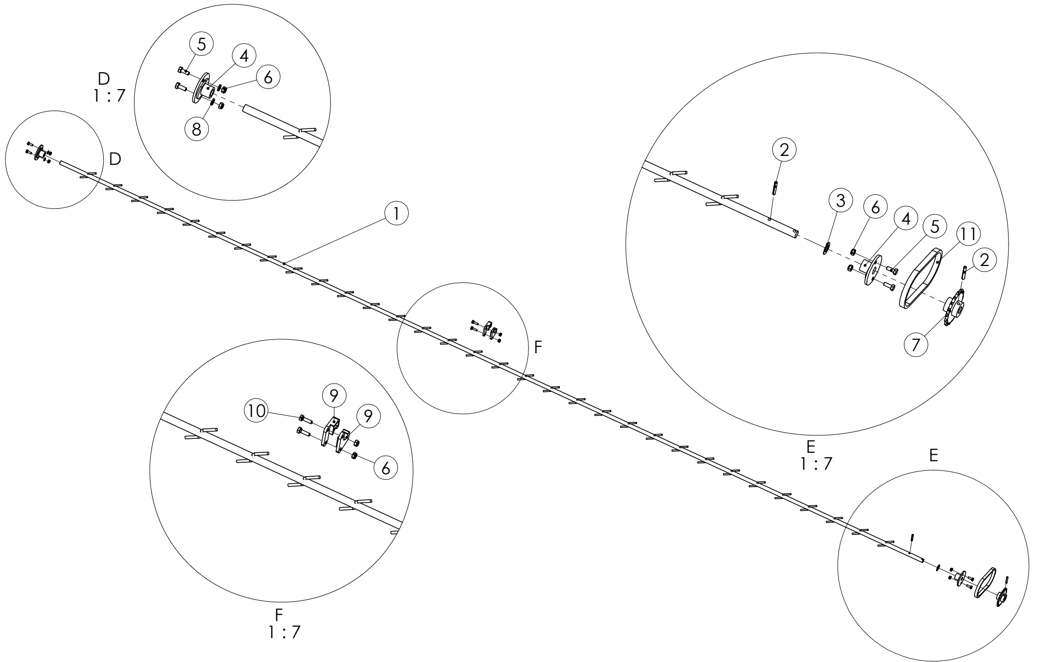
99106603 Agitator shaft for grass feed box
