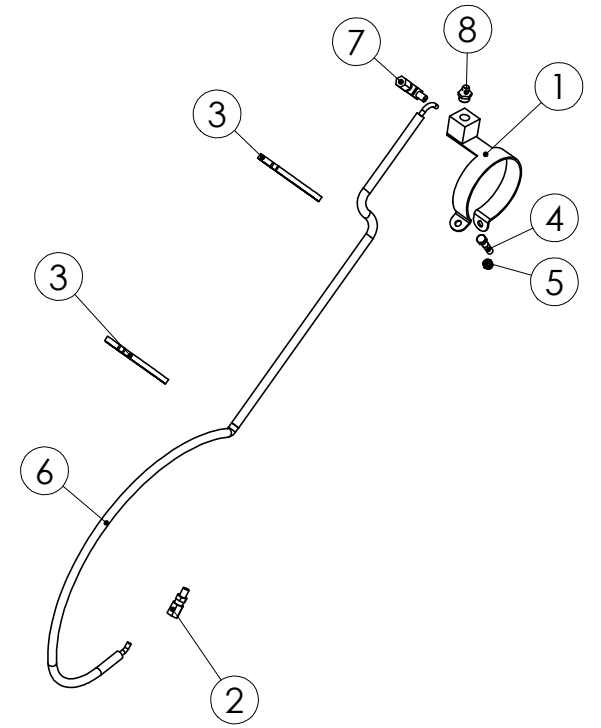
99140703 Grease nipple
