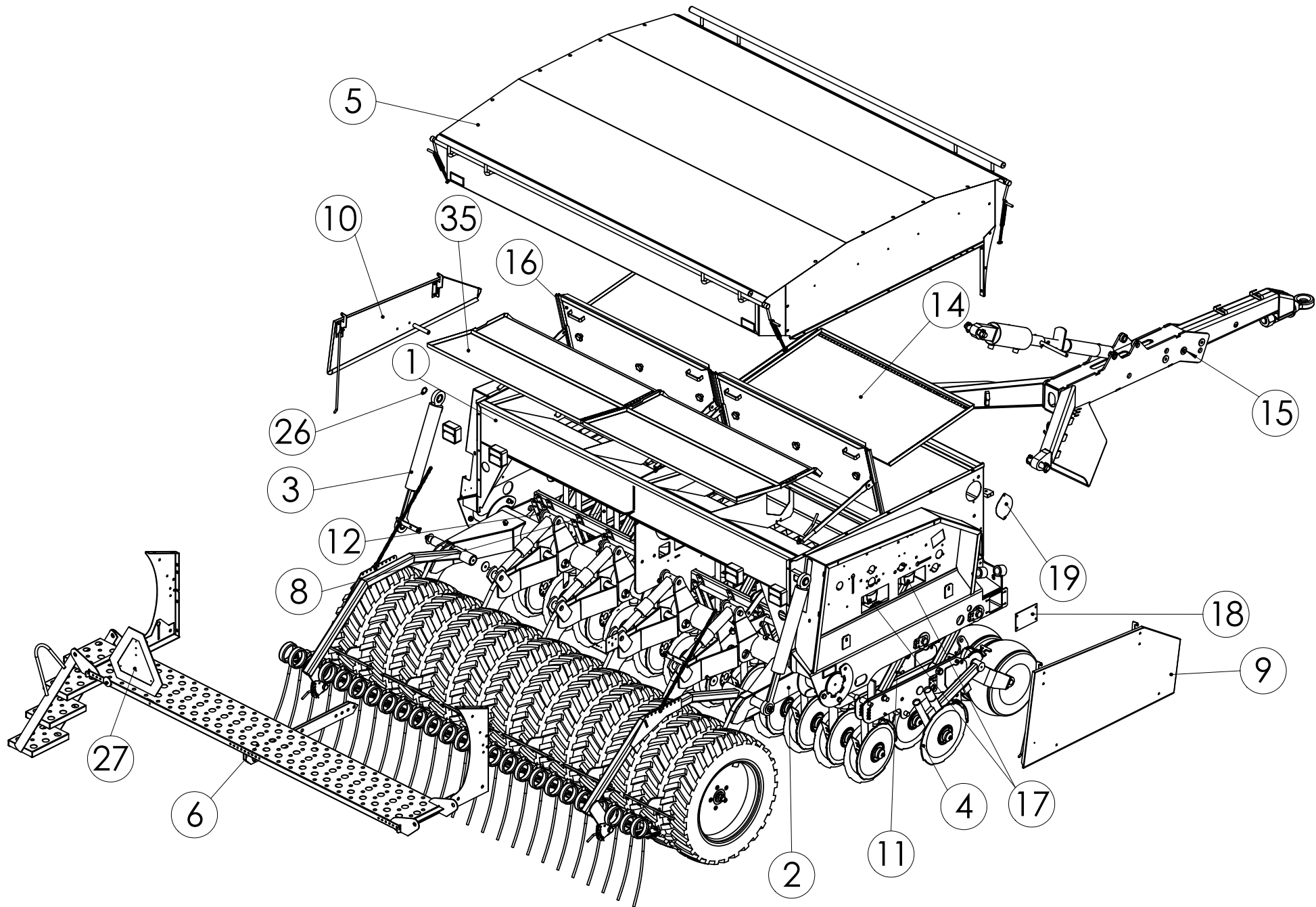
98286601 NOVACOMBI 3000
