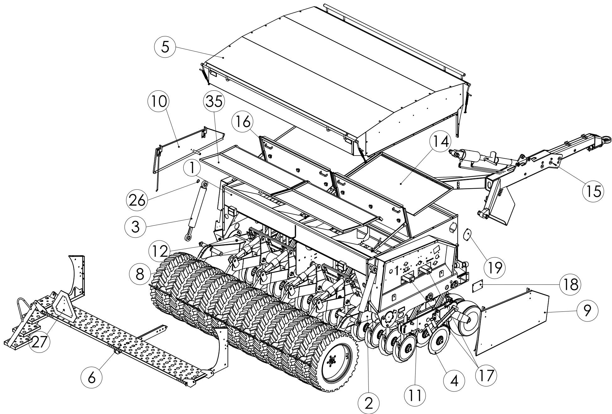
98286601 NOVACOMBI 3000
