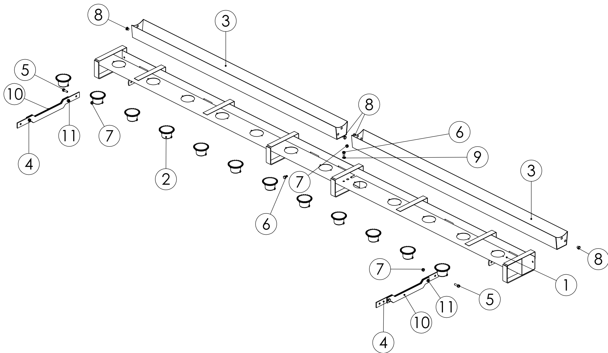
99154402 LANNOITEHYLLY JC 3000
