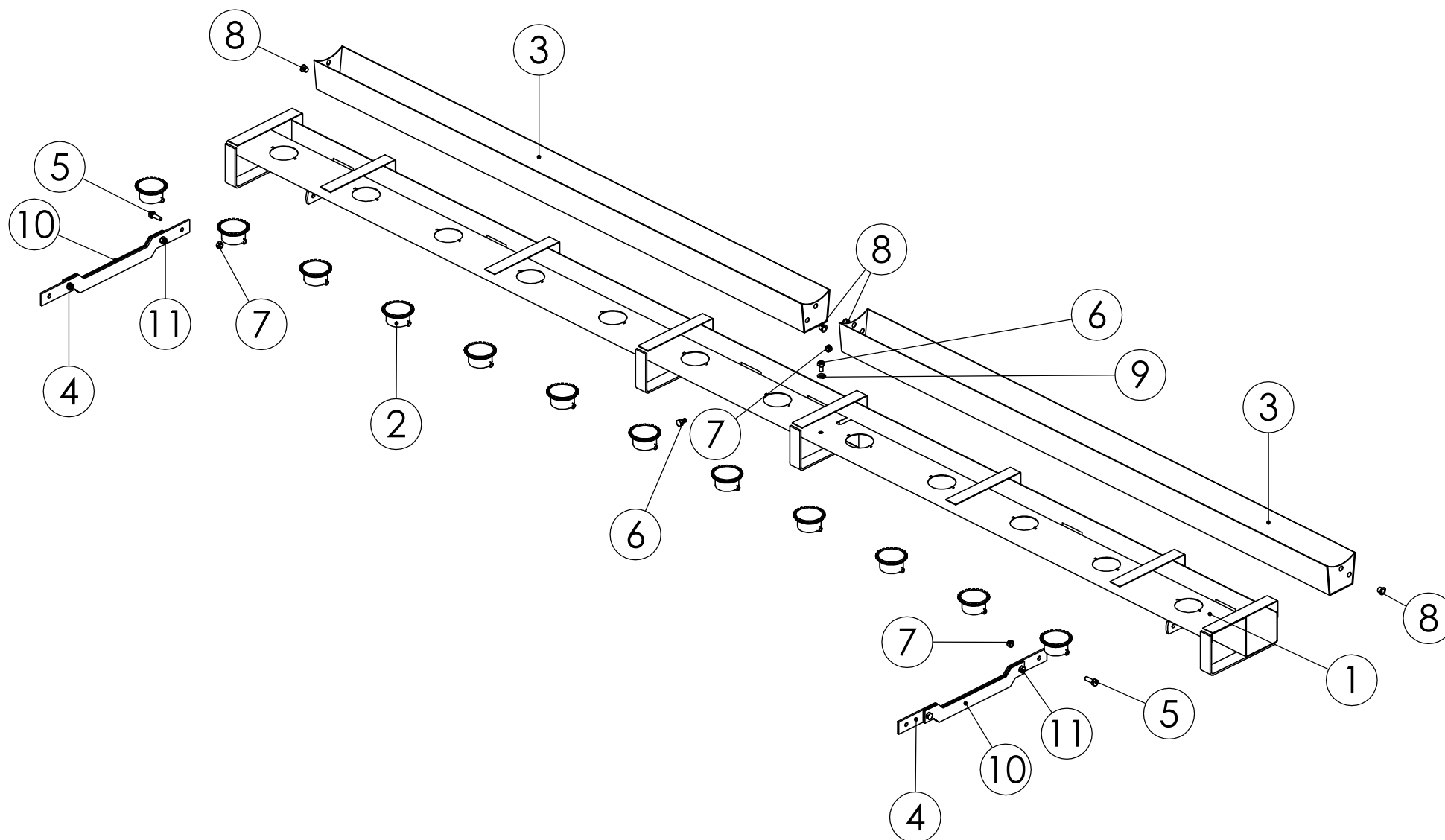
98828902 LANNOITEHYLLY JC 3000
