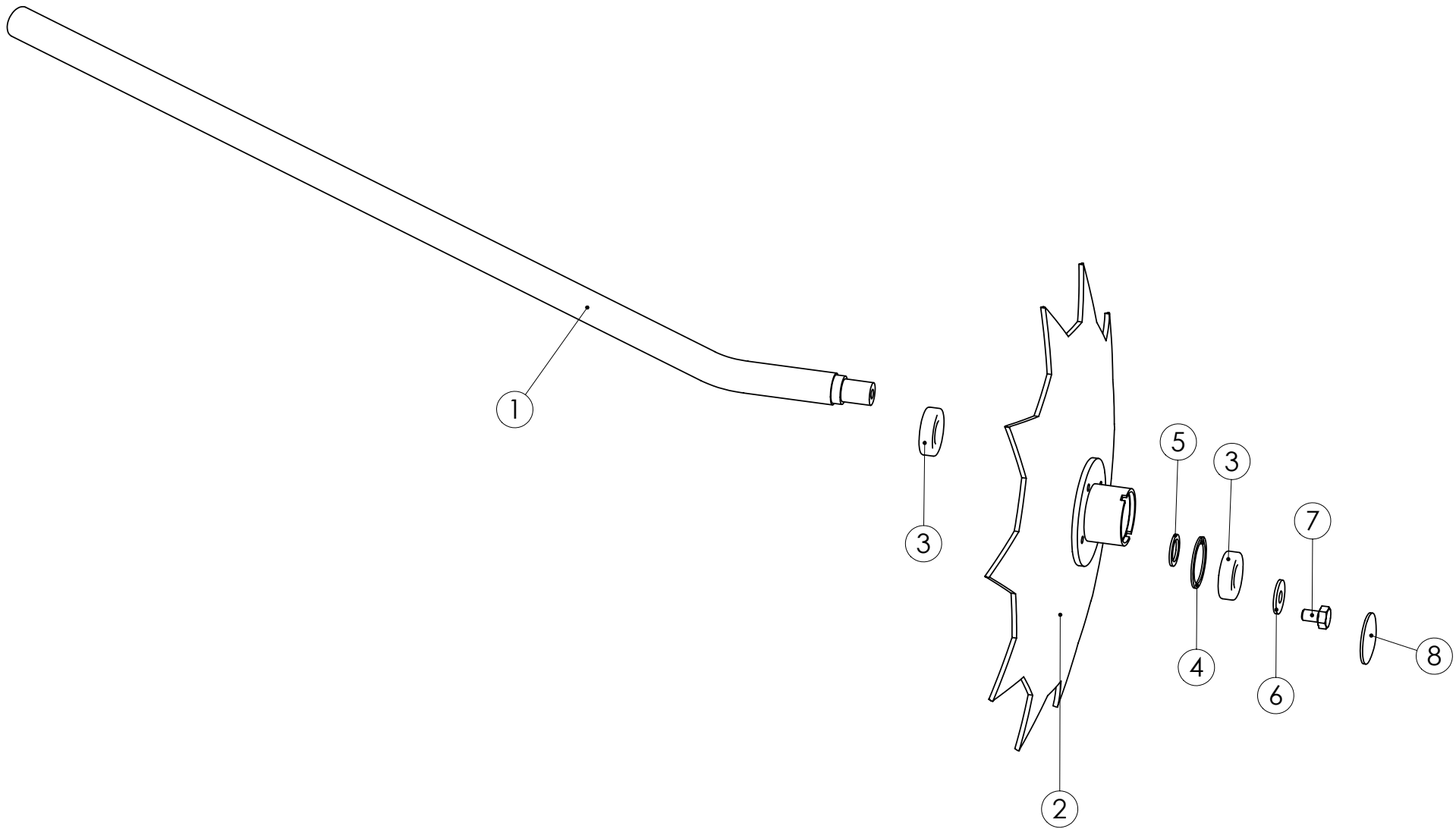
98594303 LAUTANEN+VARSI
