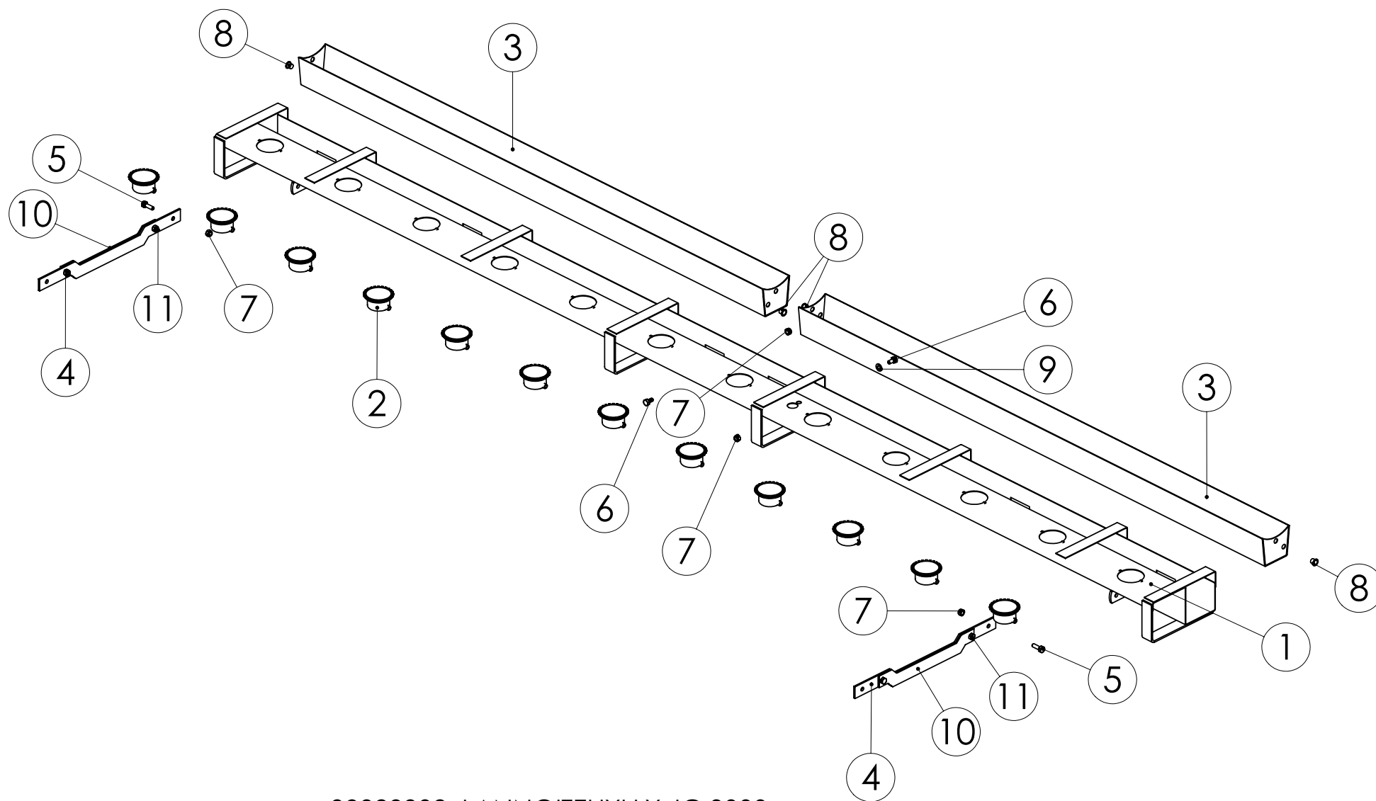
98828902 LANNOTEHYLLY JC 3000
