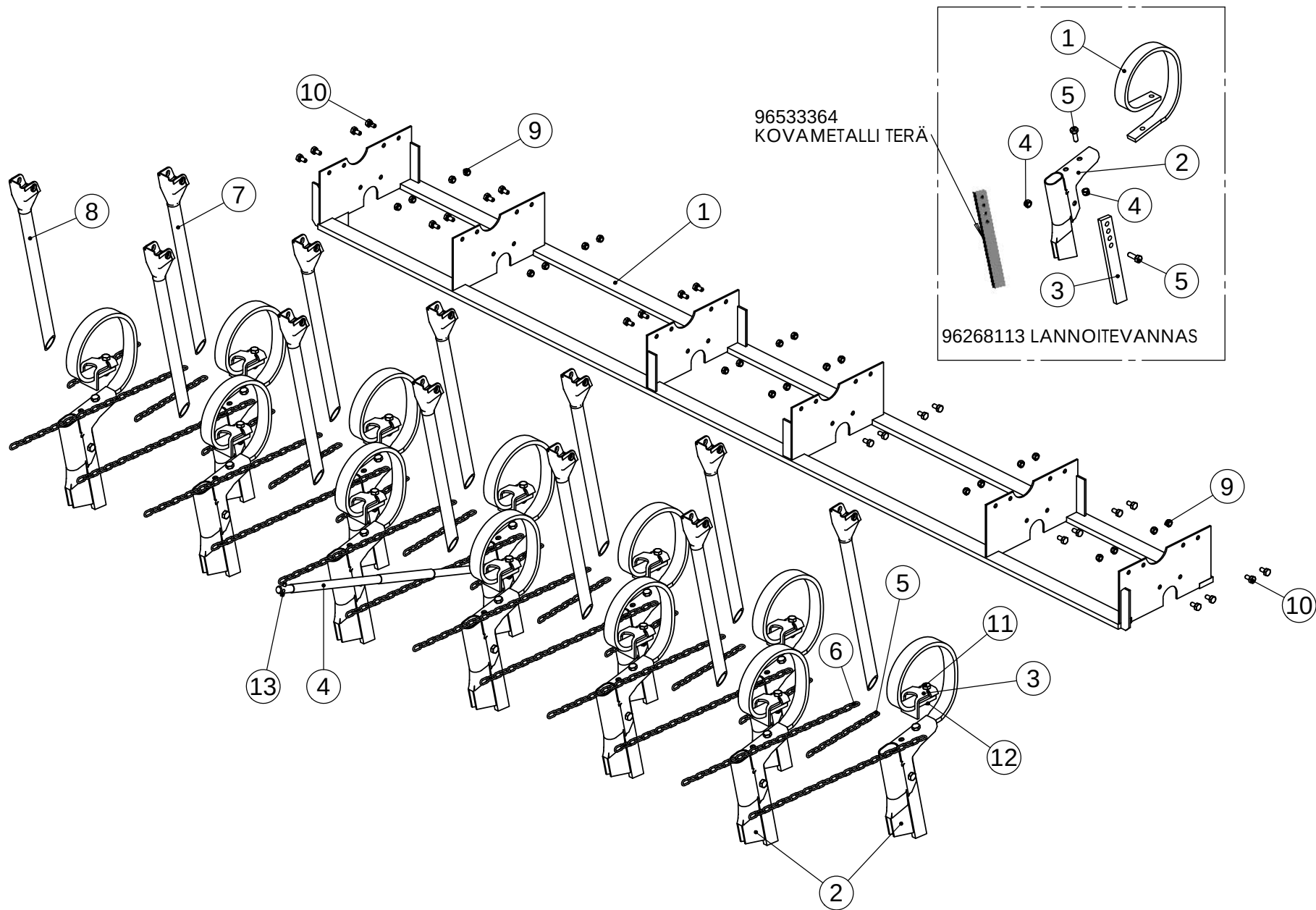
98835502 S-PIKKIRUNKO
