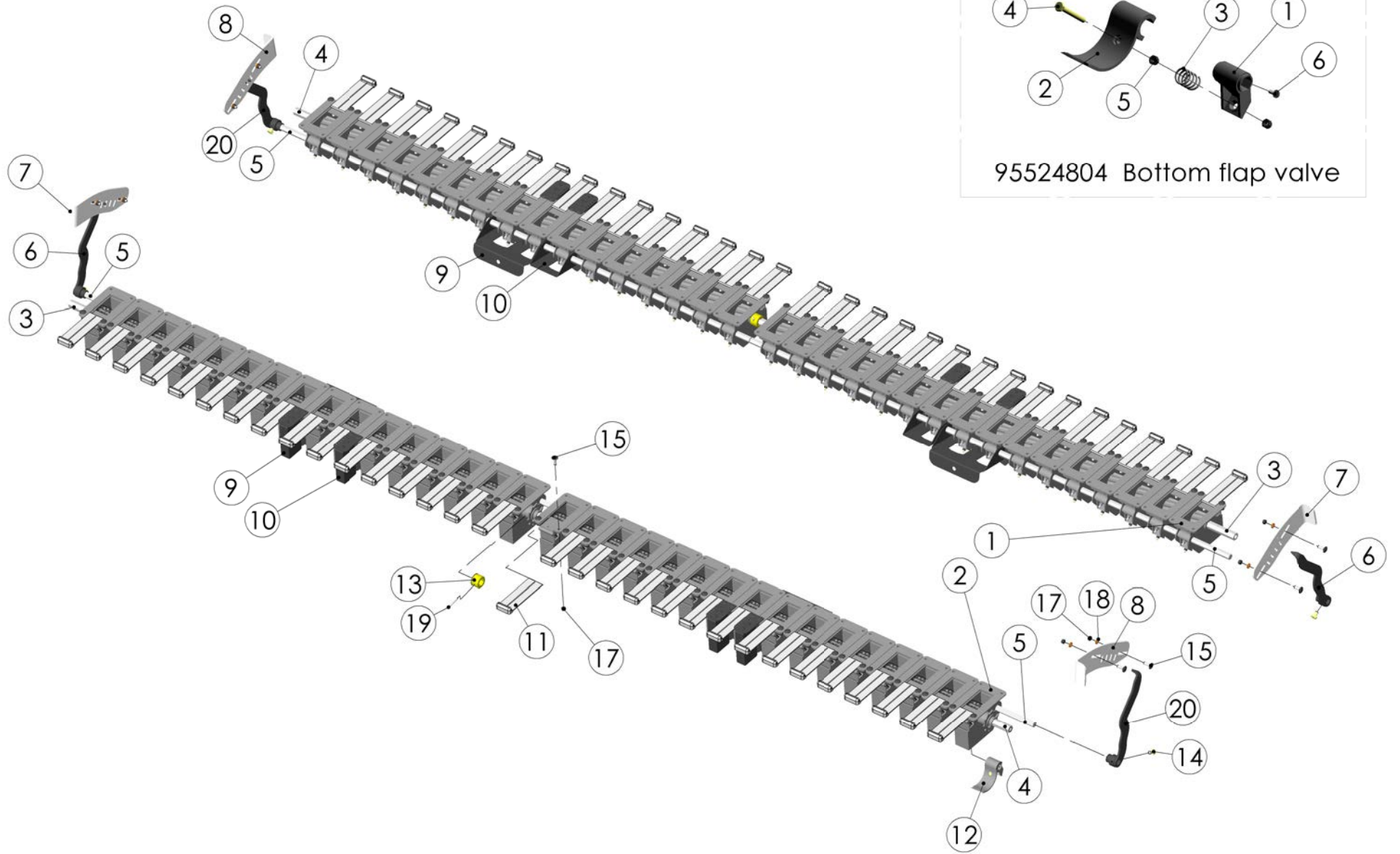
99097302 Feeding mechanism
