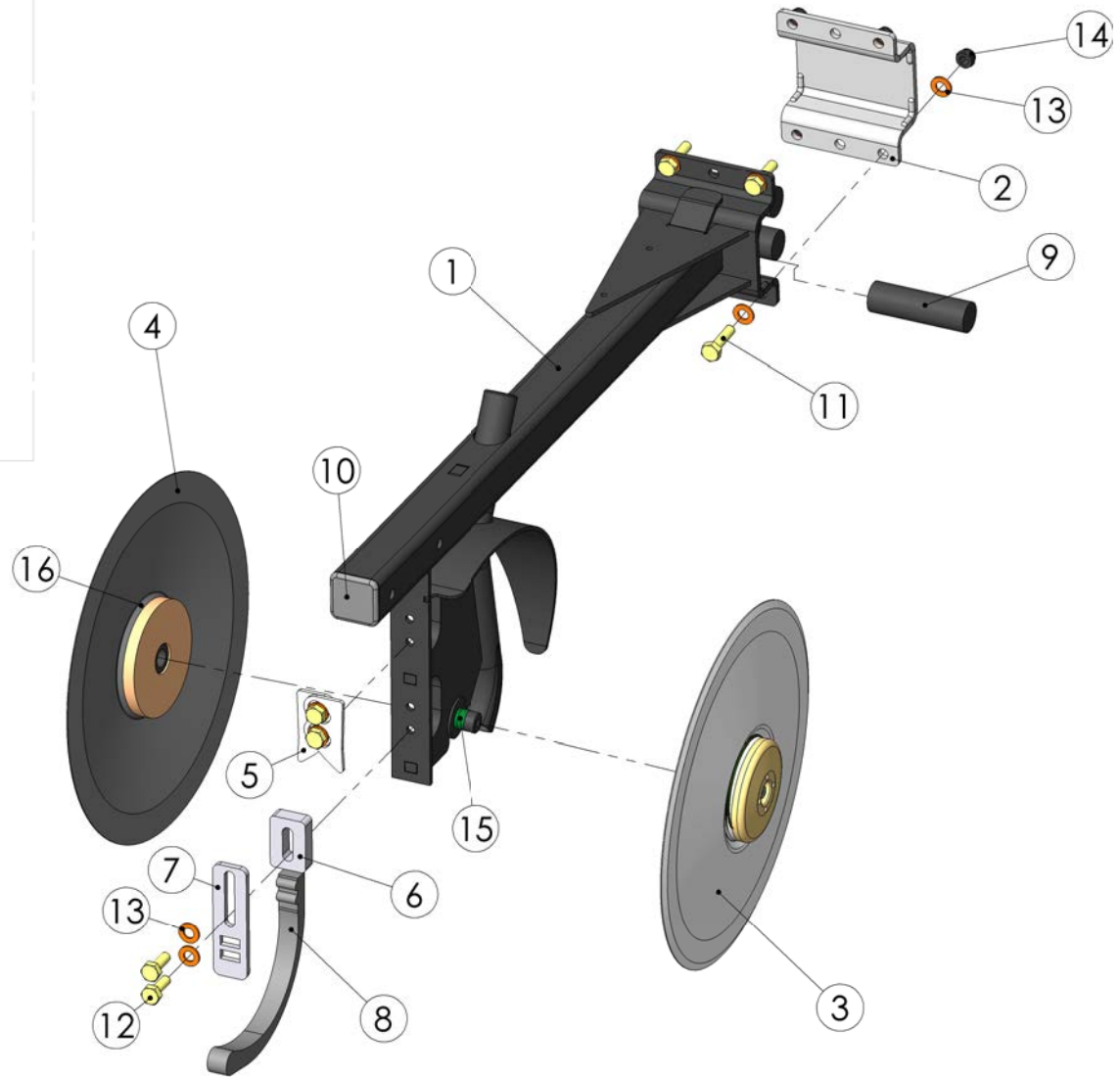
99173403 Coulter rear central
