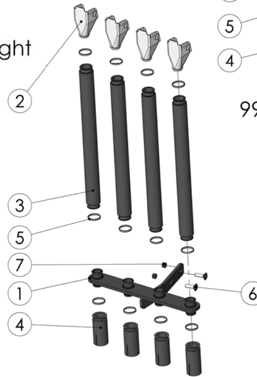
99170003 Tubes left
