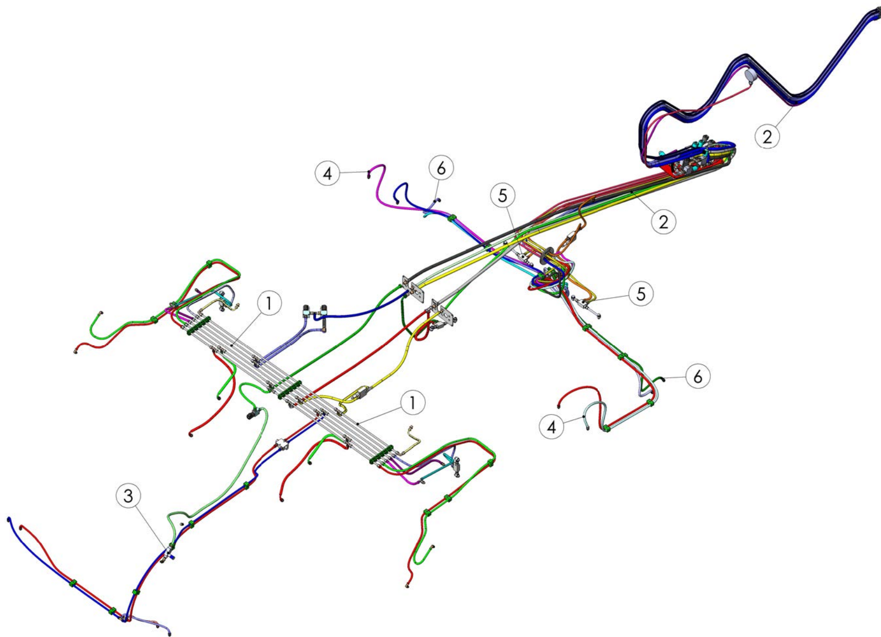
99212201 Hydraulic
