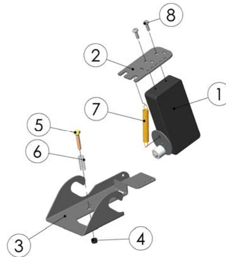
99175803 Stop motion
