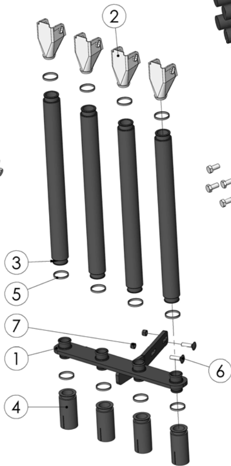
99170003 Tubes left
