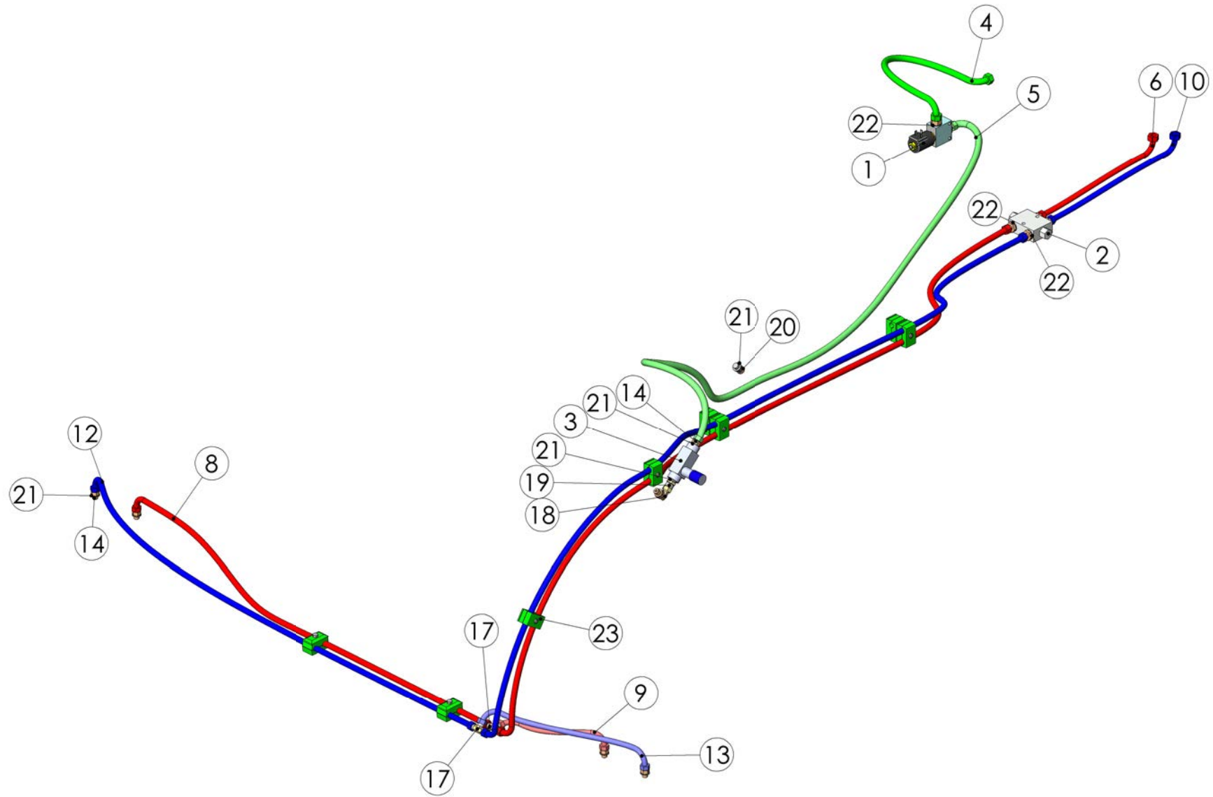
99191603 Hydraulic rear harrow
