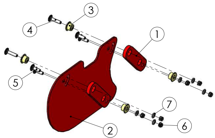
99208503 Skimmer right
