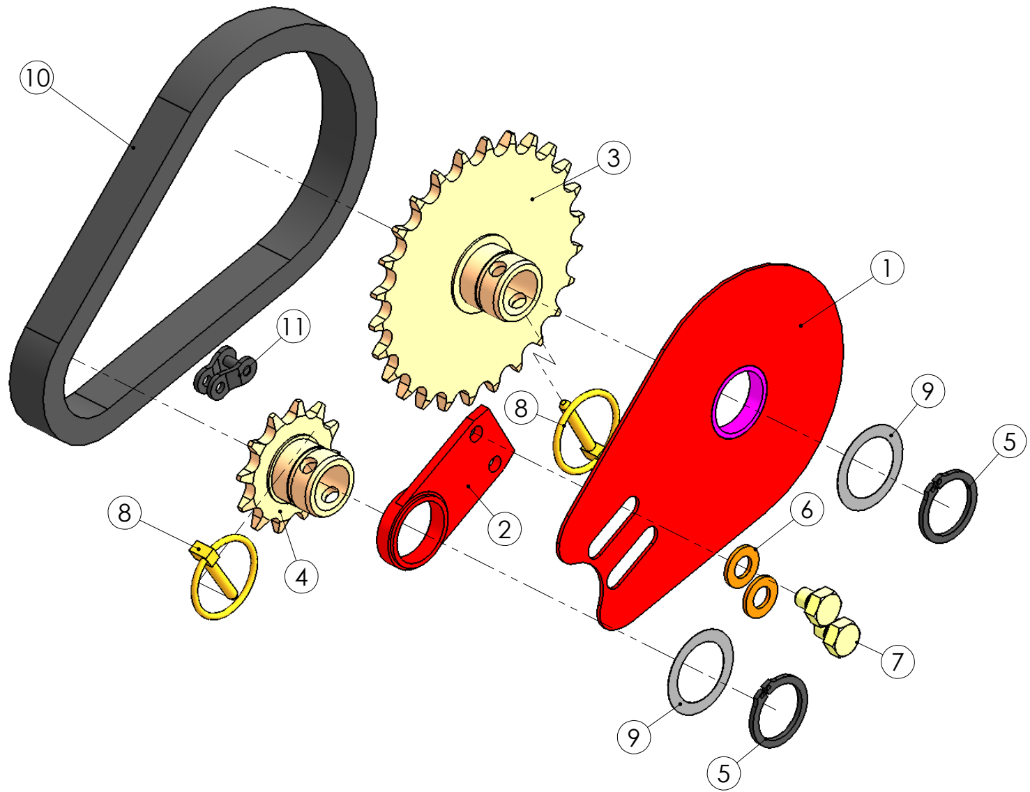
99169403 Transmission cassette
