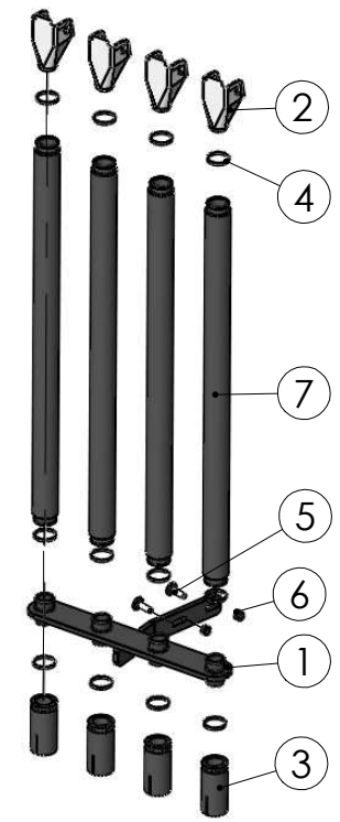
99171303 Tubes right
