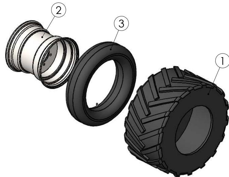
99011403 Tyre right 420/55-17
