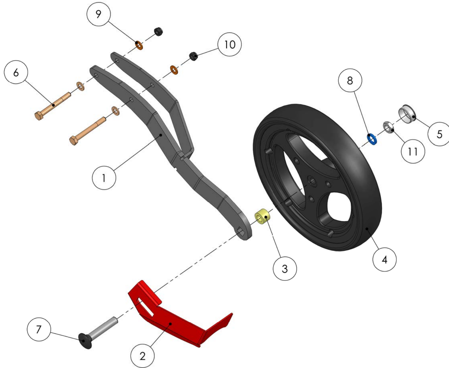
99212503 Traversing wheel
