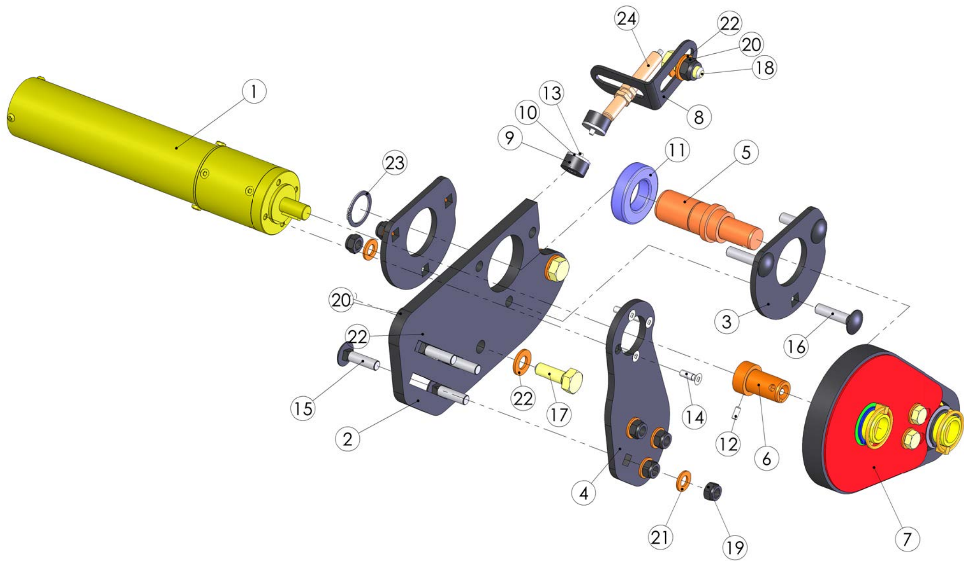
99170703 Motor right
