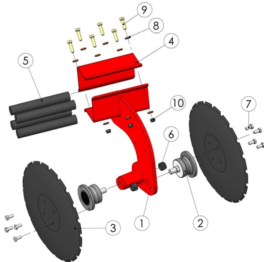
99119703 Arms right
