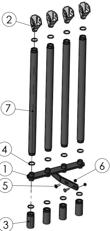
99171203 Tubes left
