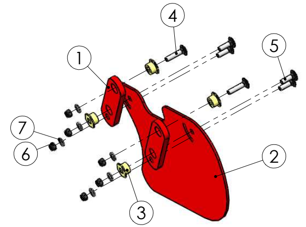
99208403 Skimmer left
