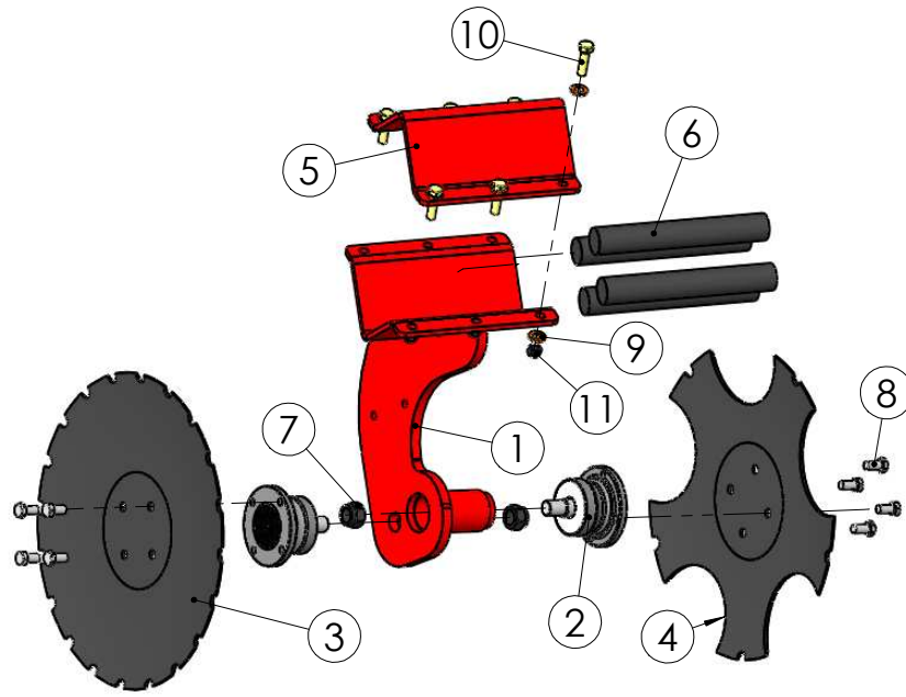
99170903 Arms right
