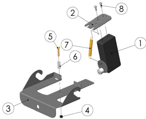
99175703 Stop motion
