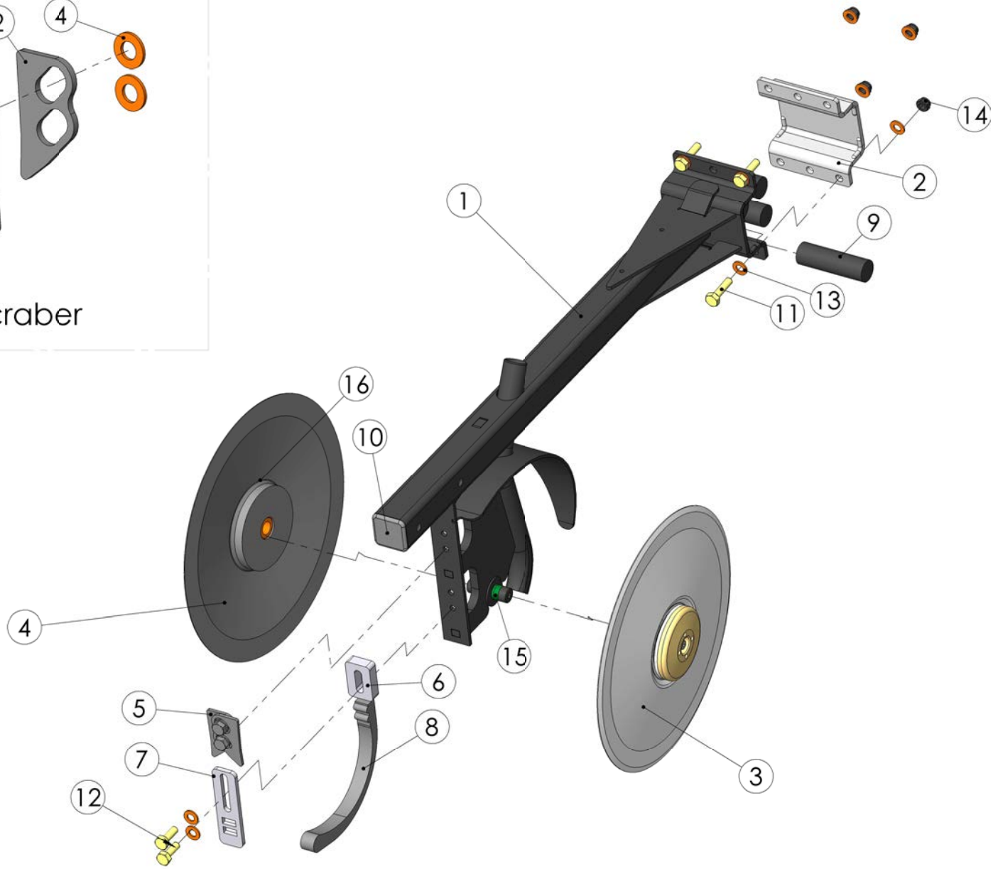
99163003 Coulter rear
