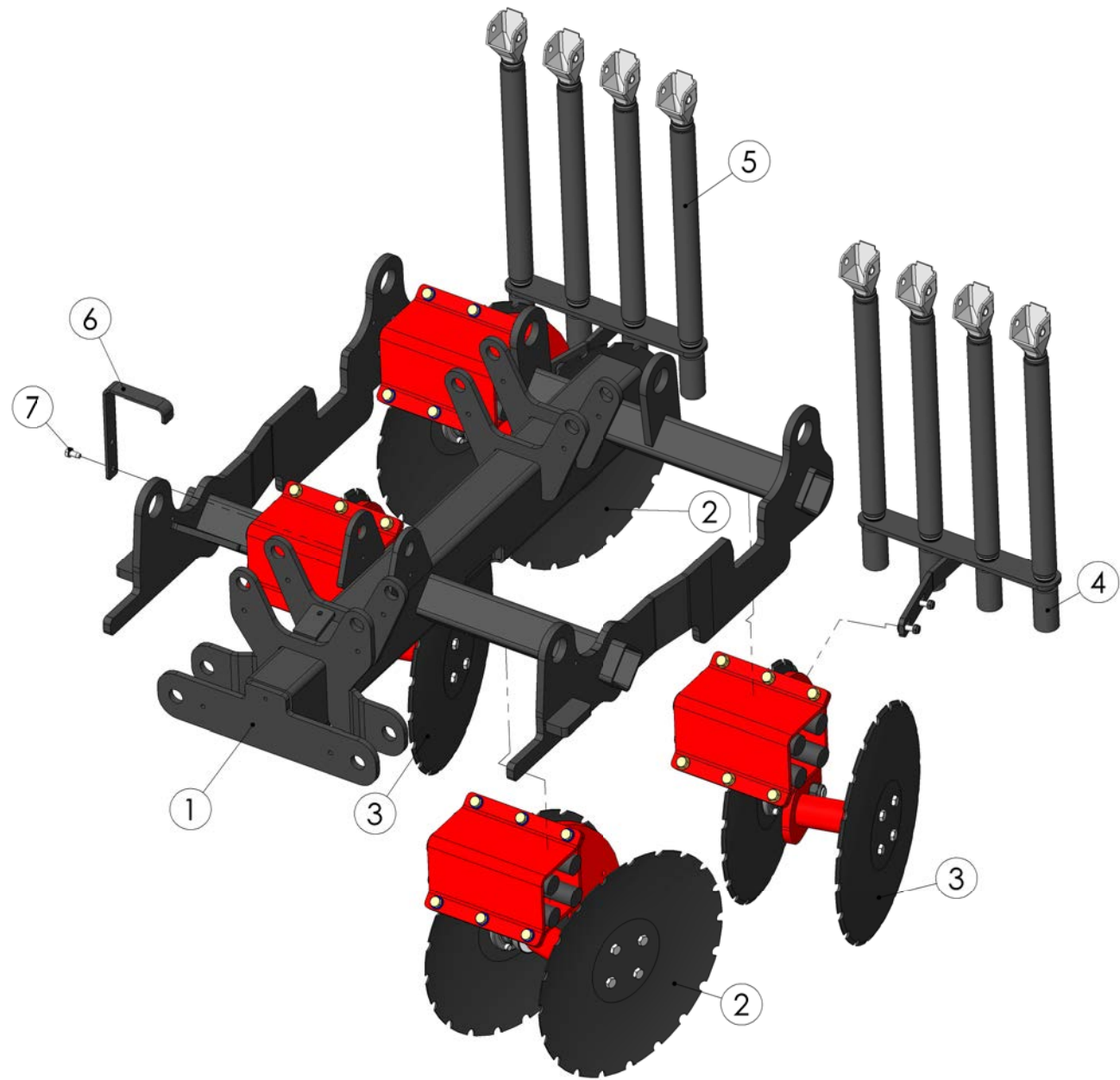
99169002 Central frame
