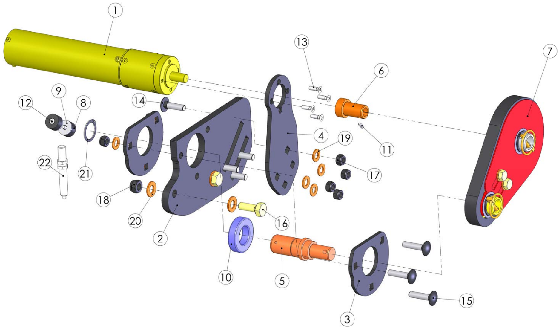
99170603 Feeding motor left
