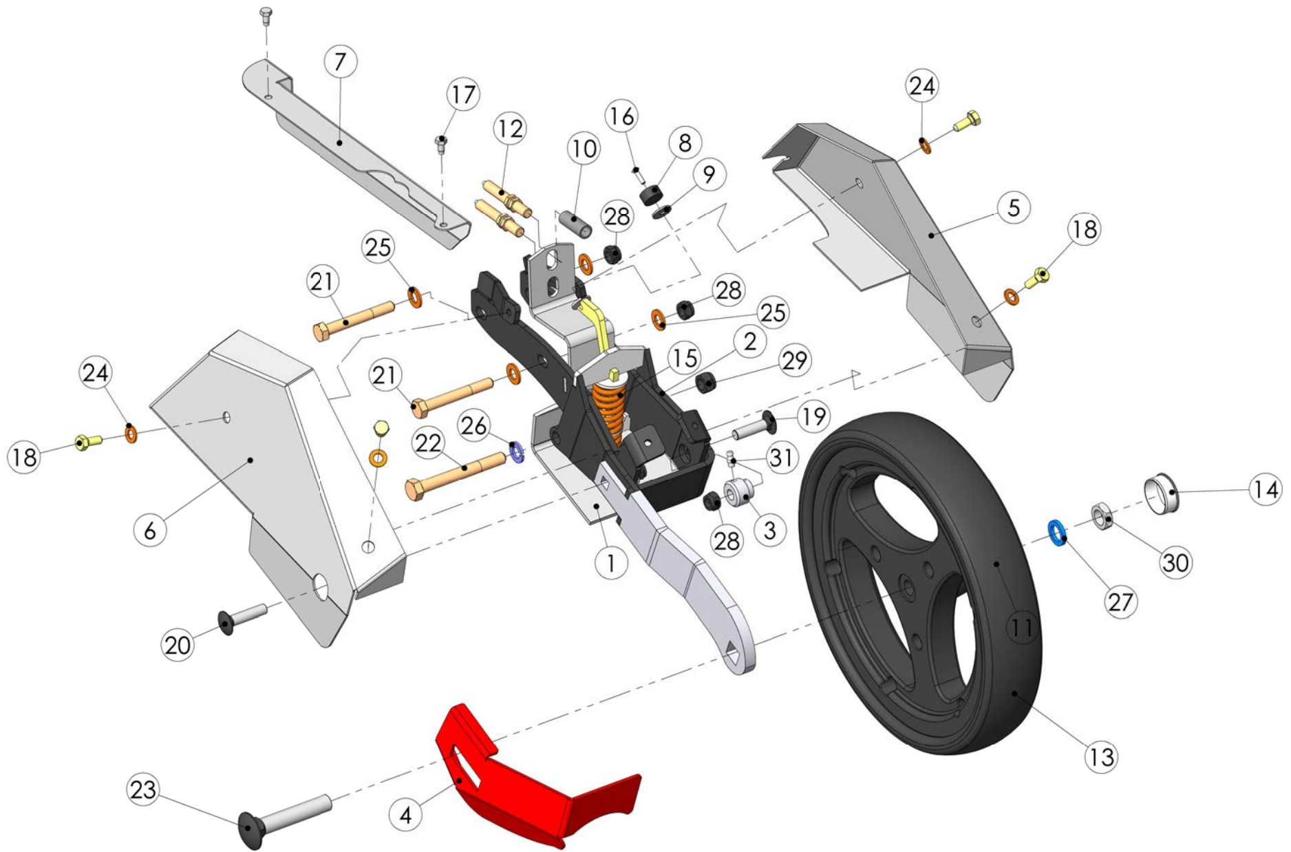
99212603 Traversing wheel
