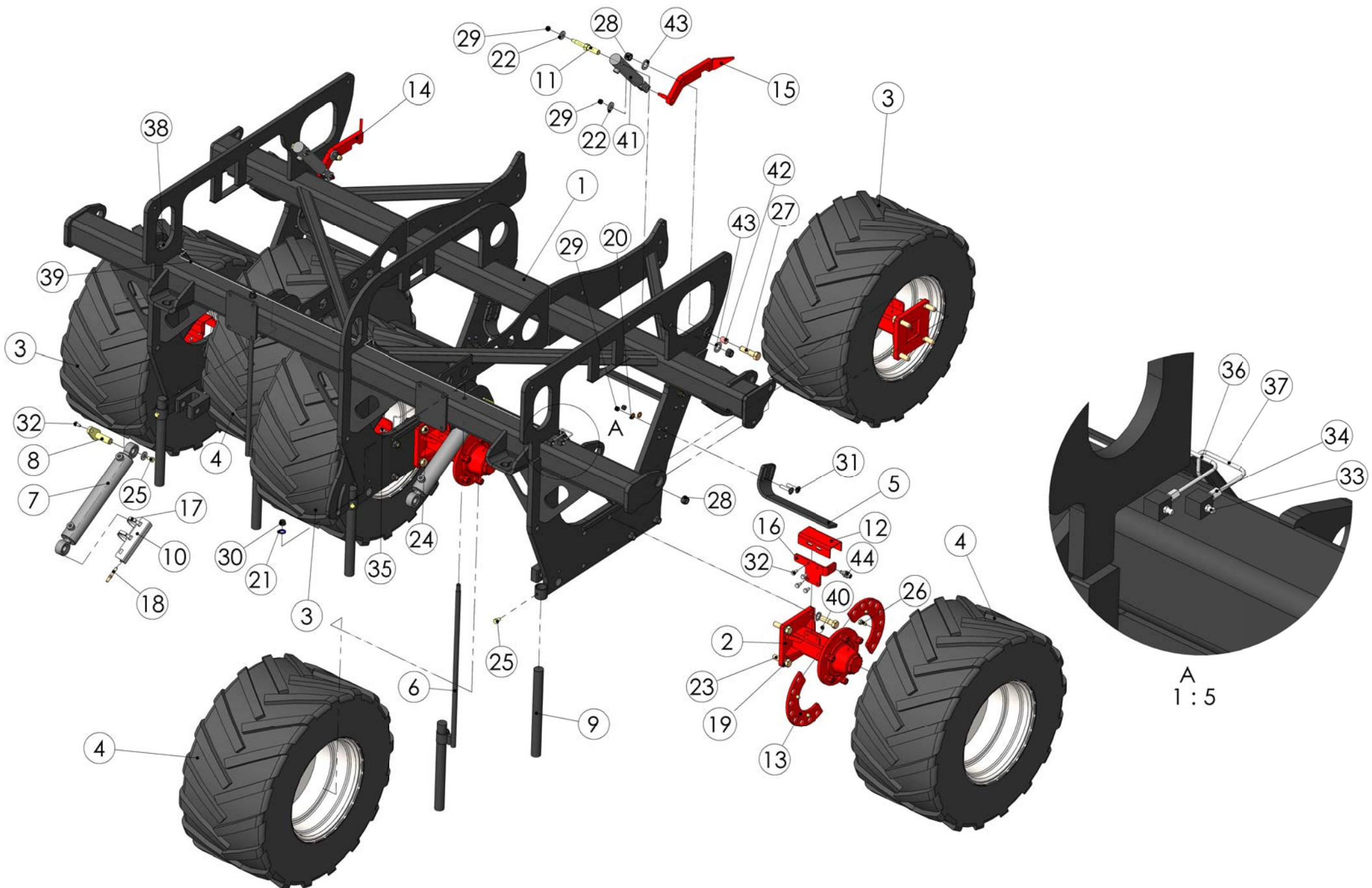
99062202 Wheel set
