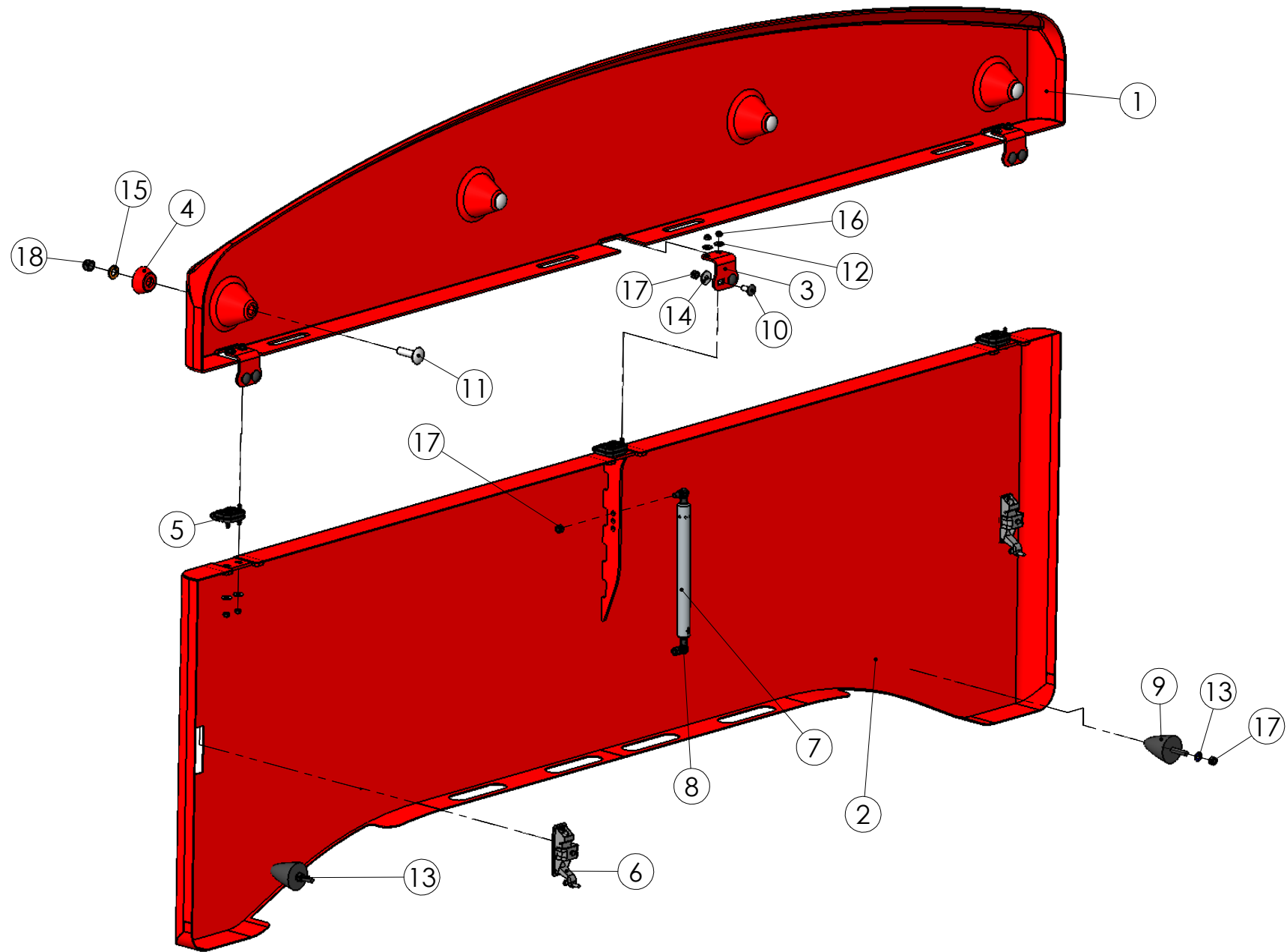
99147602 End cover
