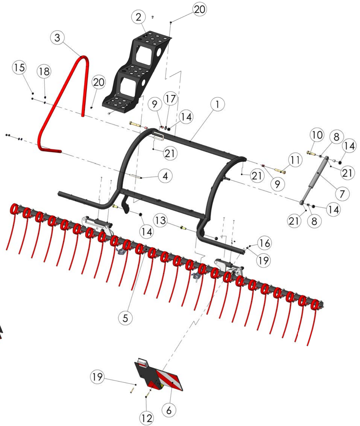
99182302 Rear harrow
