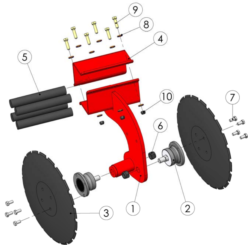
99119703 Arms right
