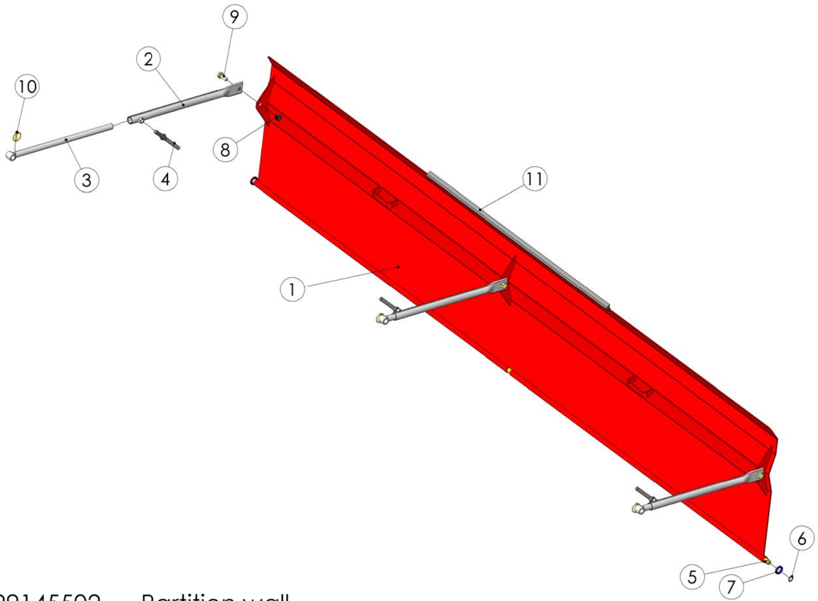
99145502 Partition wall
