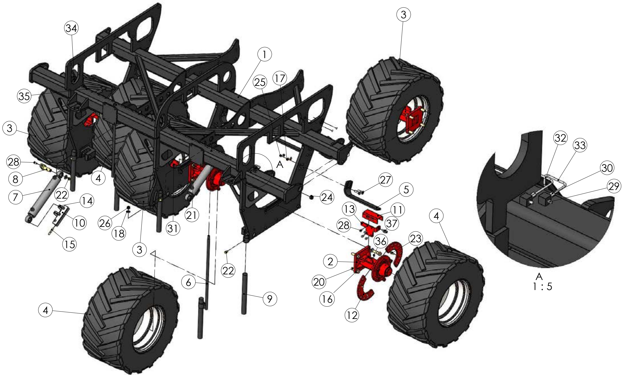
99224002 Wheel set
