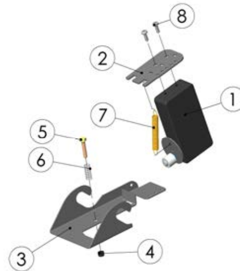
99175803 Stop motion
