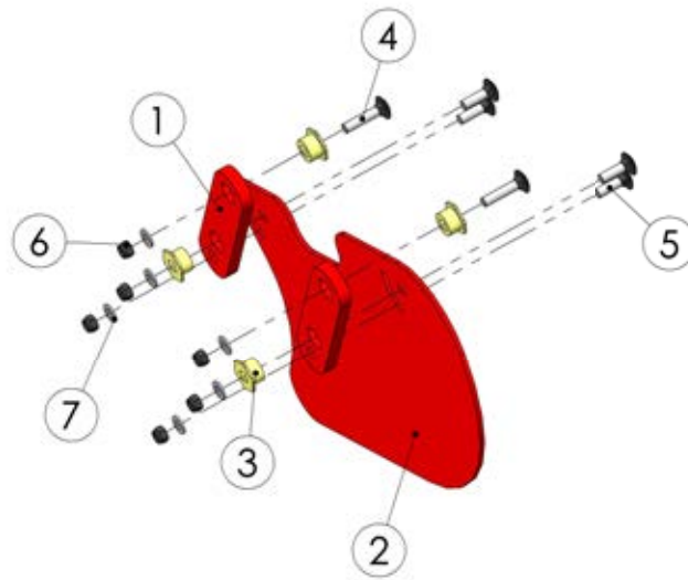
99208403 Skimmer left
