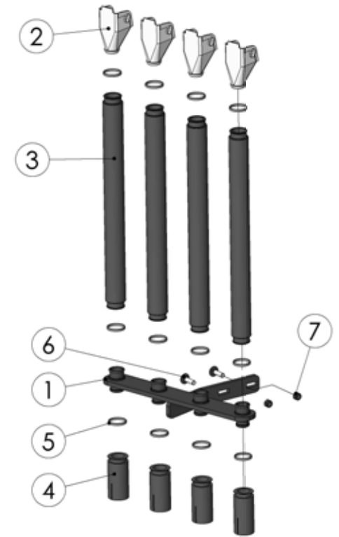
99170103 Tubes right
