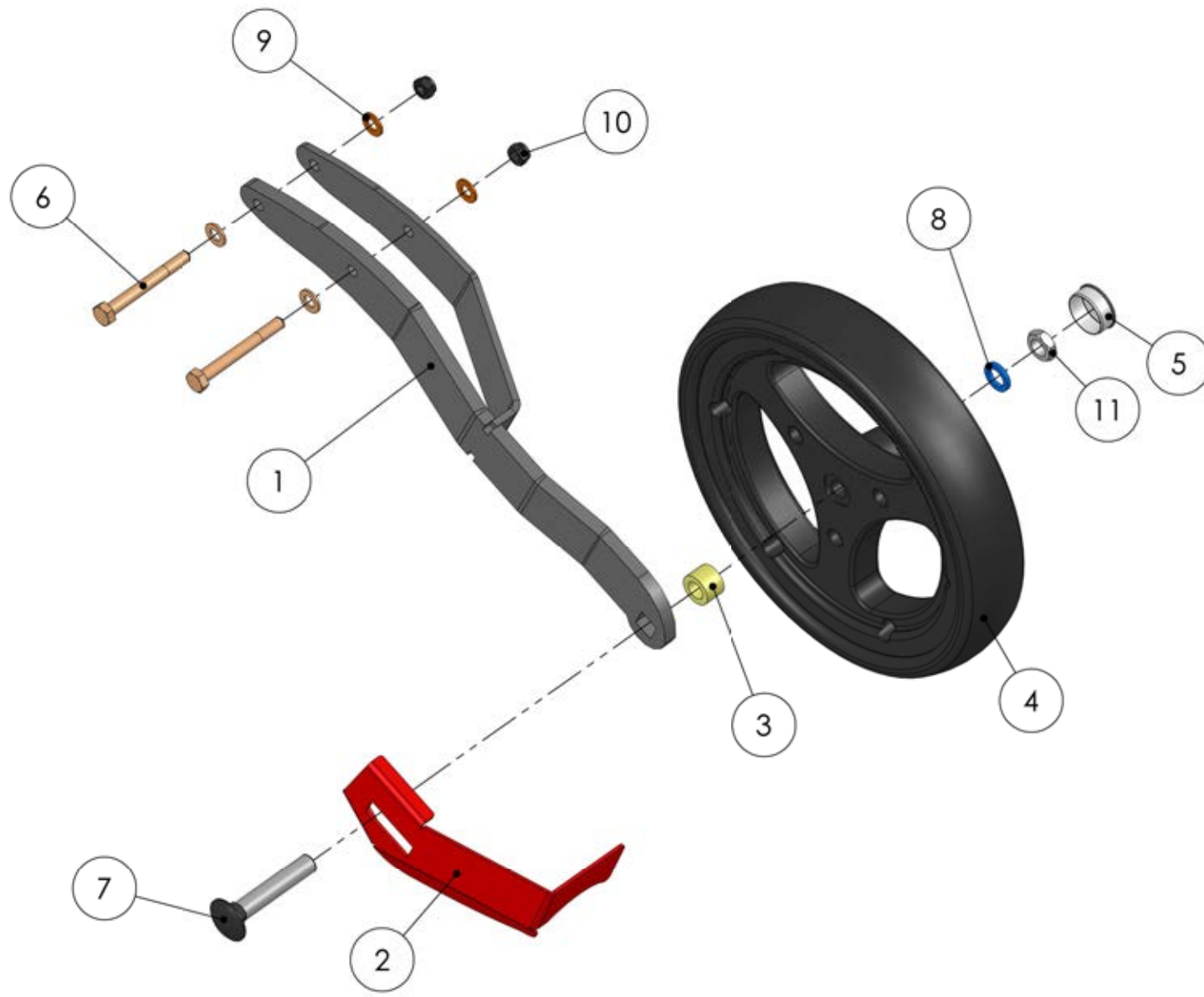
99212503 Traversing wheel
