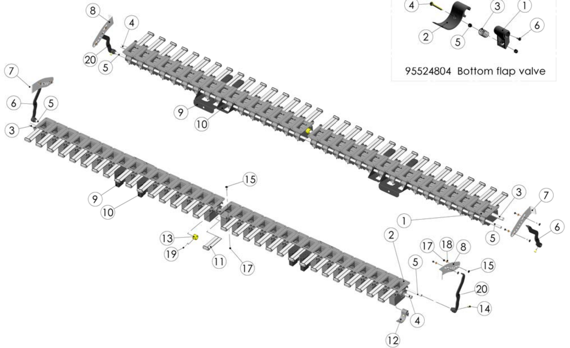
99097302 Feeding mechanism
