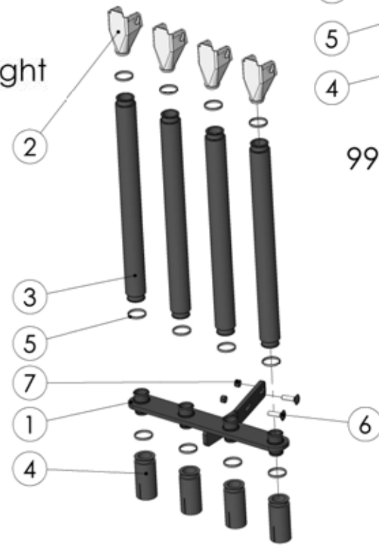
99170003 Tubes left
