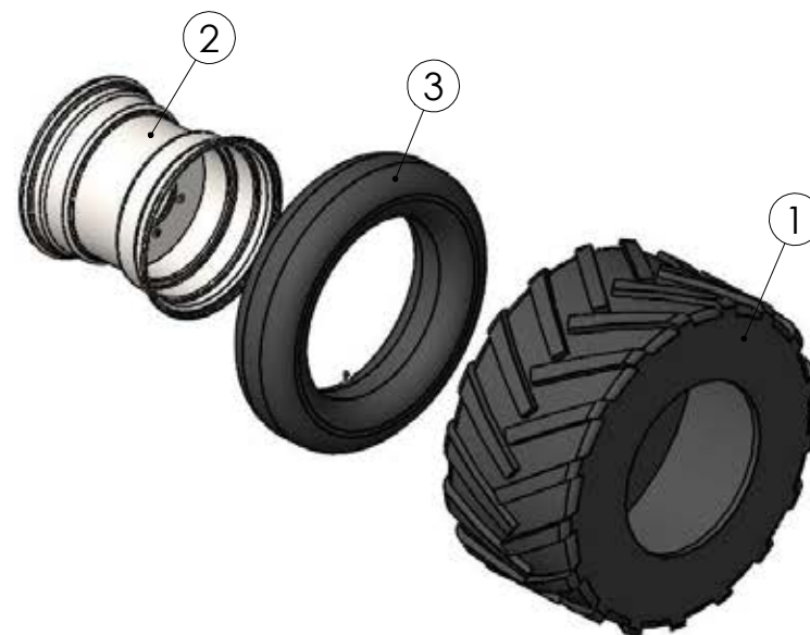
99011403 Tyre right 420/55-17
