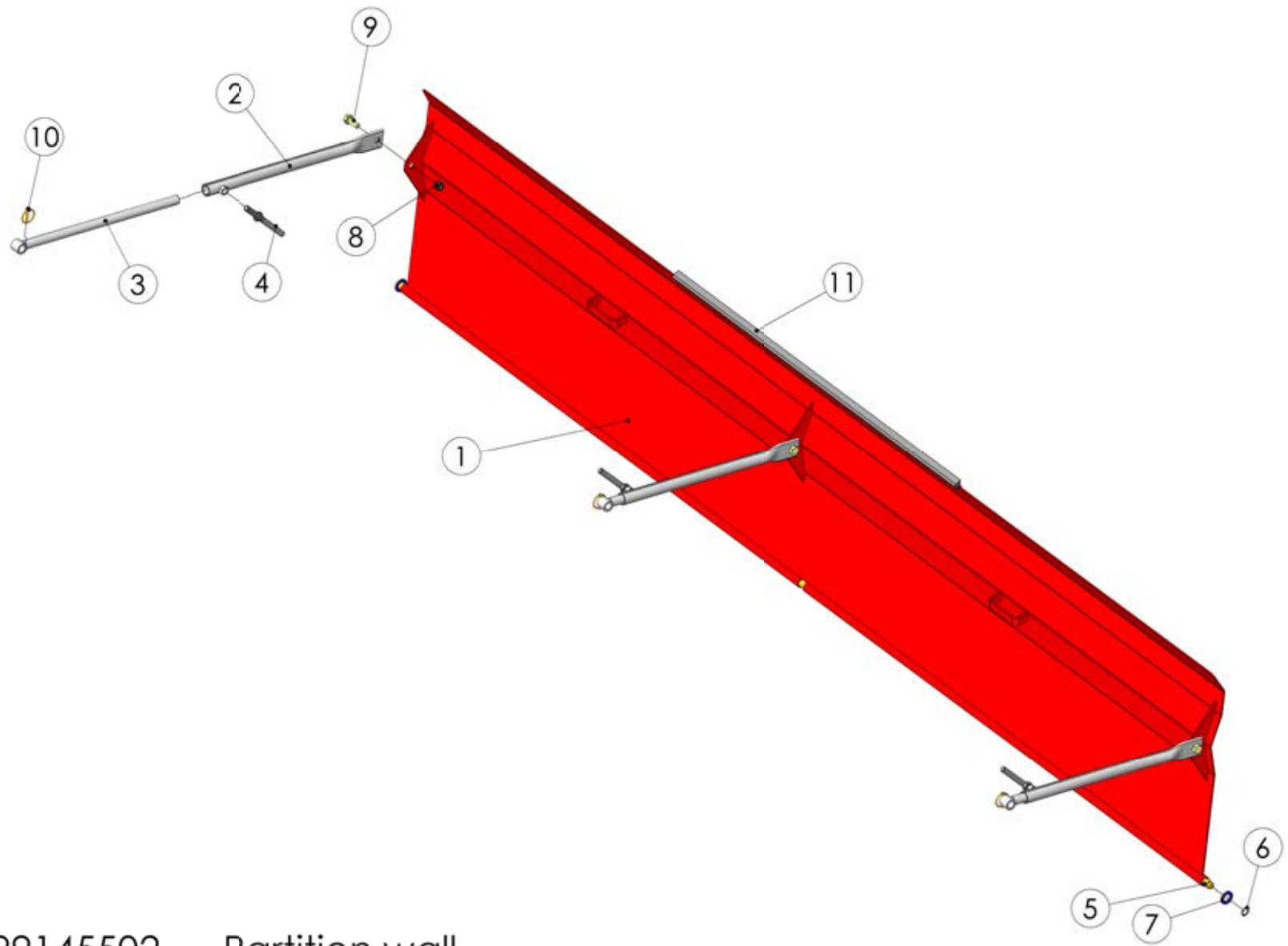
99145502 Partition wall
