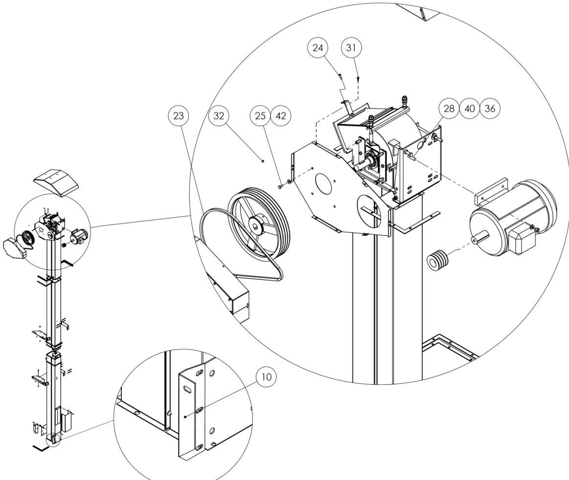
DETAIL G SCALE 1 : 5
