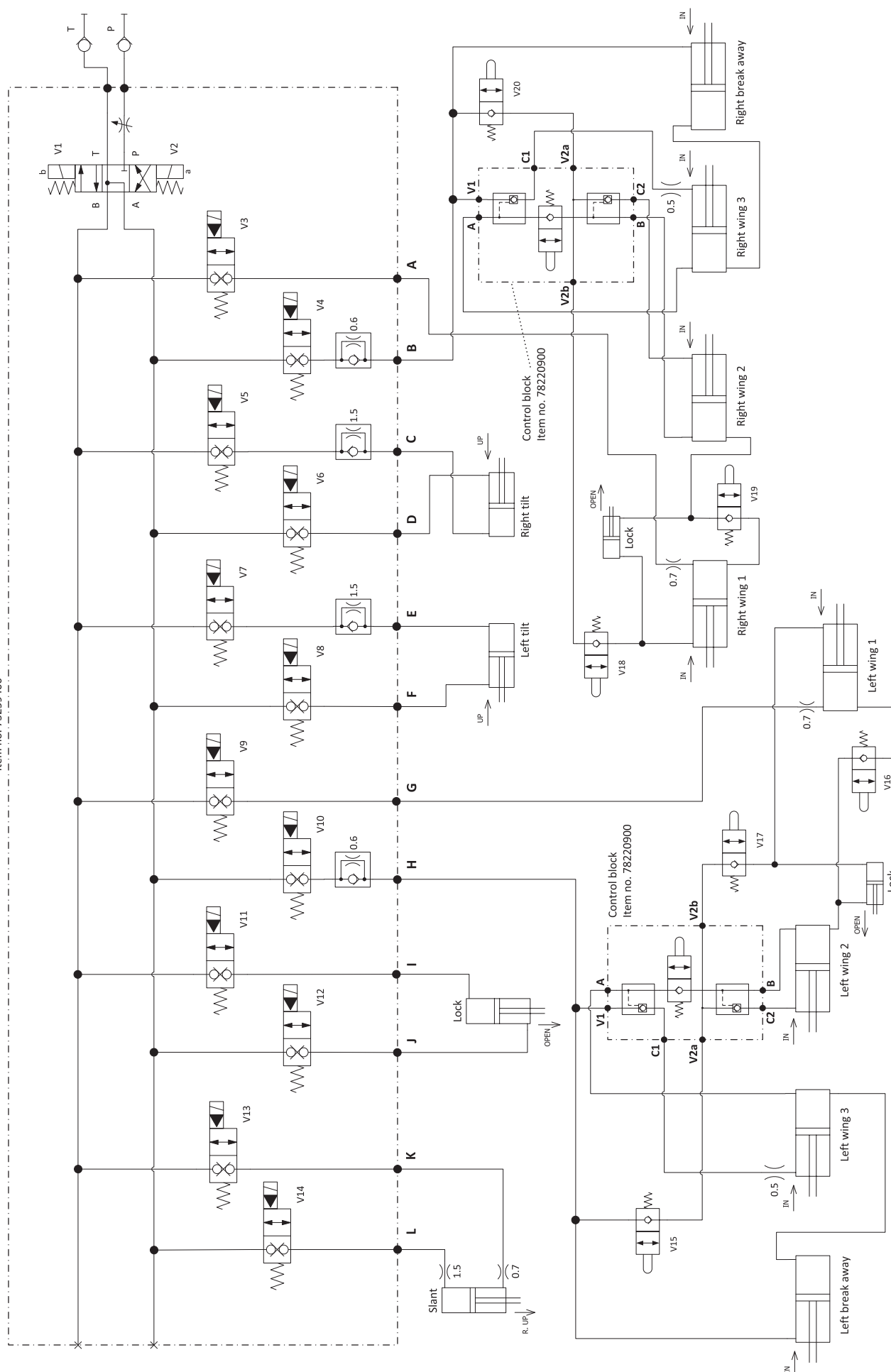
Hydraulic block in the boom centre Item no. 73259400
