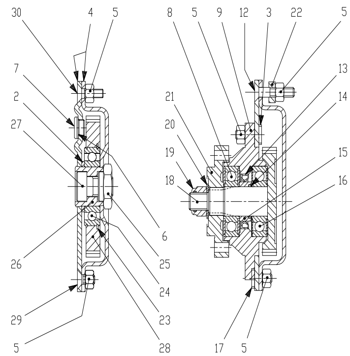
Sec. B-B
