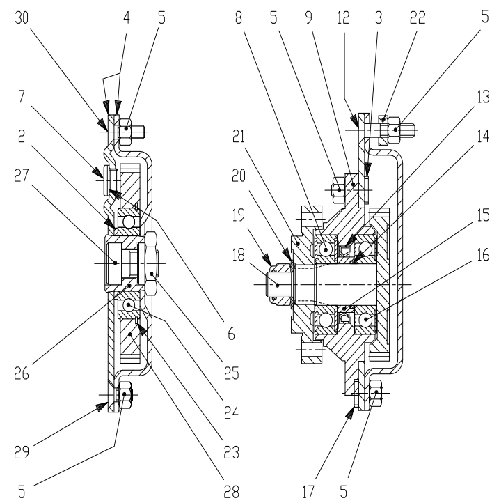
Sec. B-B
