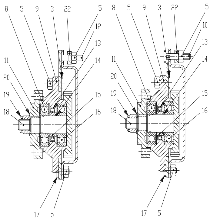
Sec. D-D
